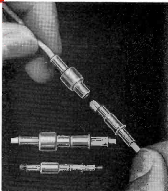
Above: Type A capacity 10 amps., and Type B capacity 5 amps. (both shown actual size)
