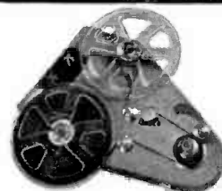
TURNTABLE-DRIVEN TAPE REPRODUCER TL-10
