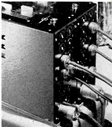
Twist-lock devices in use on a Davis portable dimmer.
